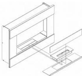
Picture 3. Glass mounting In biofireplaces Alpha, Bravo, Bravo 2, Charlie, Charlie 2, Delta, Delta 2, Golf, Quat.
